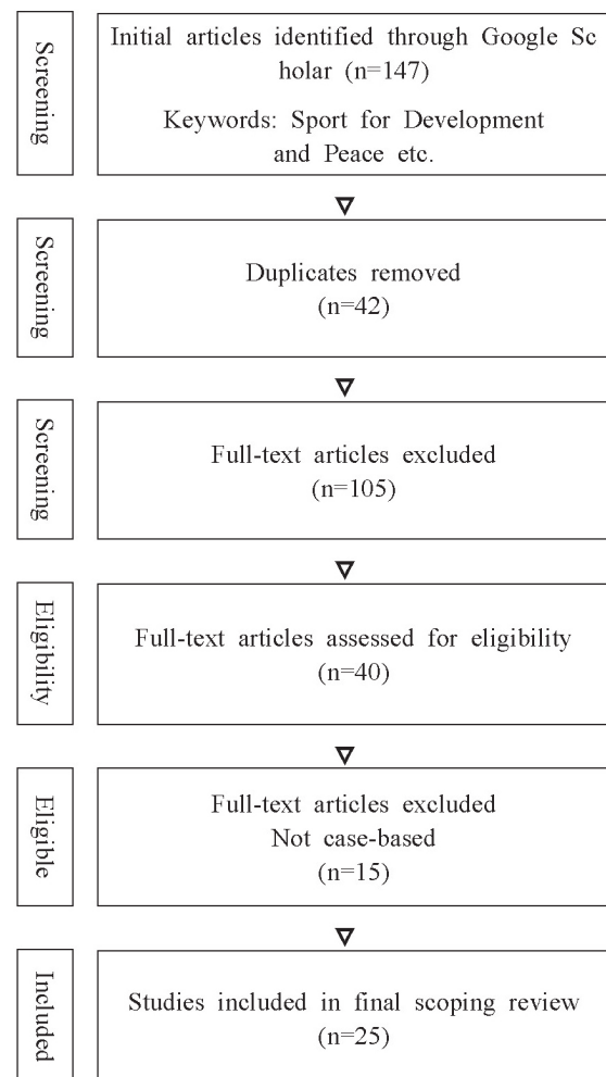
Fig. 1. PRISMA flowchart
